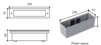
Plastic sleeve
