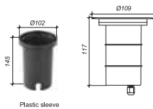
Plastic sleeve
