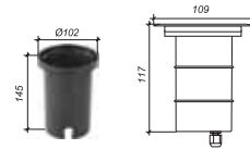
Plastic sleeve
