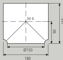
Elemento terminal Tube end
