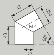
Conector angular Corner connector
