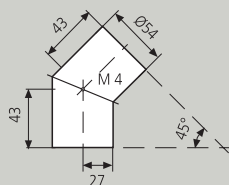
Conector angular Corner connector
