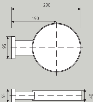
Brazo extensor Wall bracket
