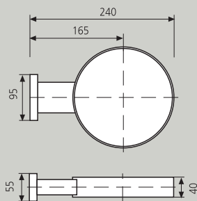
Brazo extensor Wall bracket
