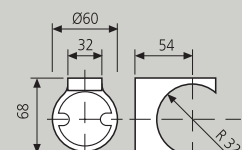
Brazo extensible Wall bracket overlapping
