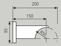
Brazo extensor extensible con pie Wall bracket overlapping with foot
