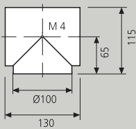
Arco 30° Bend 30°
