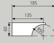
Brazo extensor extensible sin pie Wall bracket overlapping less foot
