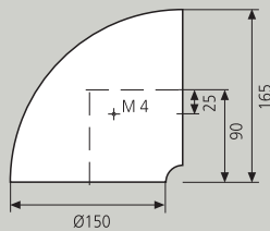
Brazo extensor Wall bracket
