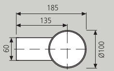
Brazo extensor sin pie Wall bracket less foot
