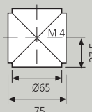
Conector triple 1 x 90^{\circ} y 2 x 135^{\circ} 3-way connector 1 x 90^{\circ} and 2 x 135^{\circ}
