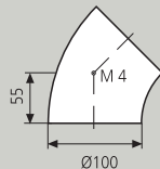
Conector triple 1 x 90° - 2 x 135° 3-way connector 1 x 90° - 2 x 135°
