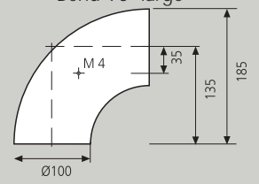
Arco 90° grande Bend 90° large
