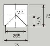
Conector triple 3 x 90^{\circ} 3-way connector 3 x 90^{\circ}
