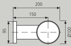
Brazo extensor con pie Wall bracket with foot
